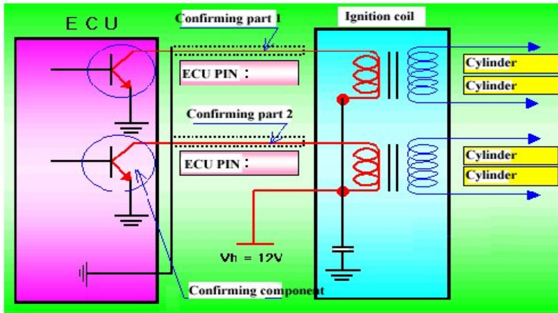
<Distributorless type circuit>
