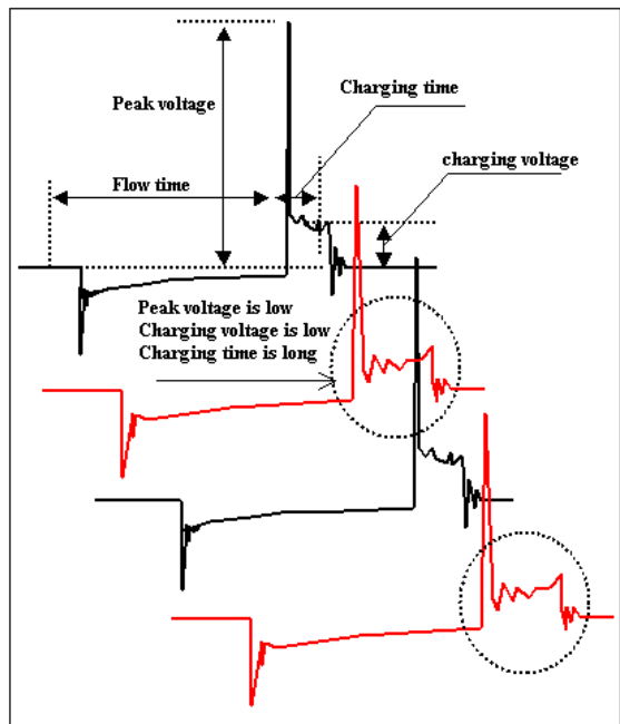
Left case: The gap of plug tip is too wide or secondary ignition system has big resistance. Right case: The gap of plug tip is too narrow or exist factor of cause inside combustion chamber as rich mixed gas or low compression ratio.
