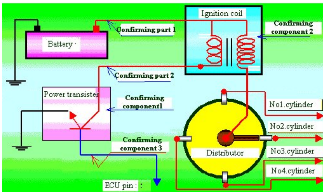
<Distributor type circuit>
