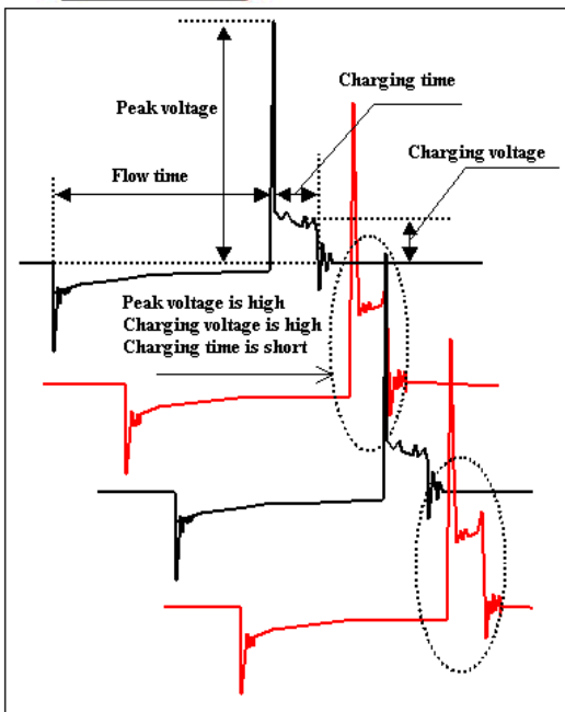
Left case: The gap of plug tip is too wide or secondary ignition system has big resistance. Right case: The gap of plug tip is too narrow or exist factor of cause inside combustion chamber as rich mixed gas or low compression ratio.
